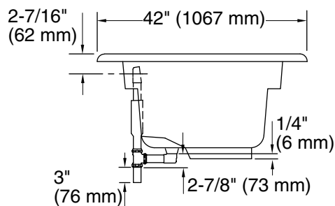
Drop-in Rim Detail
