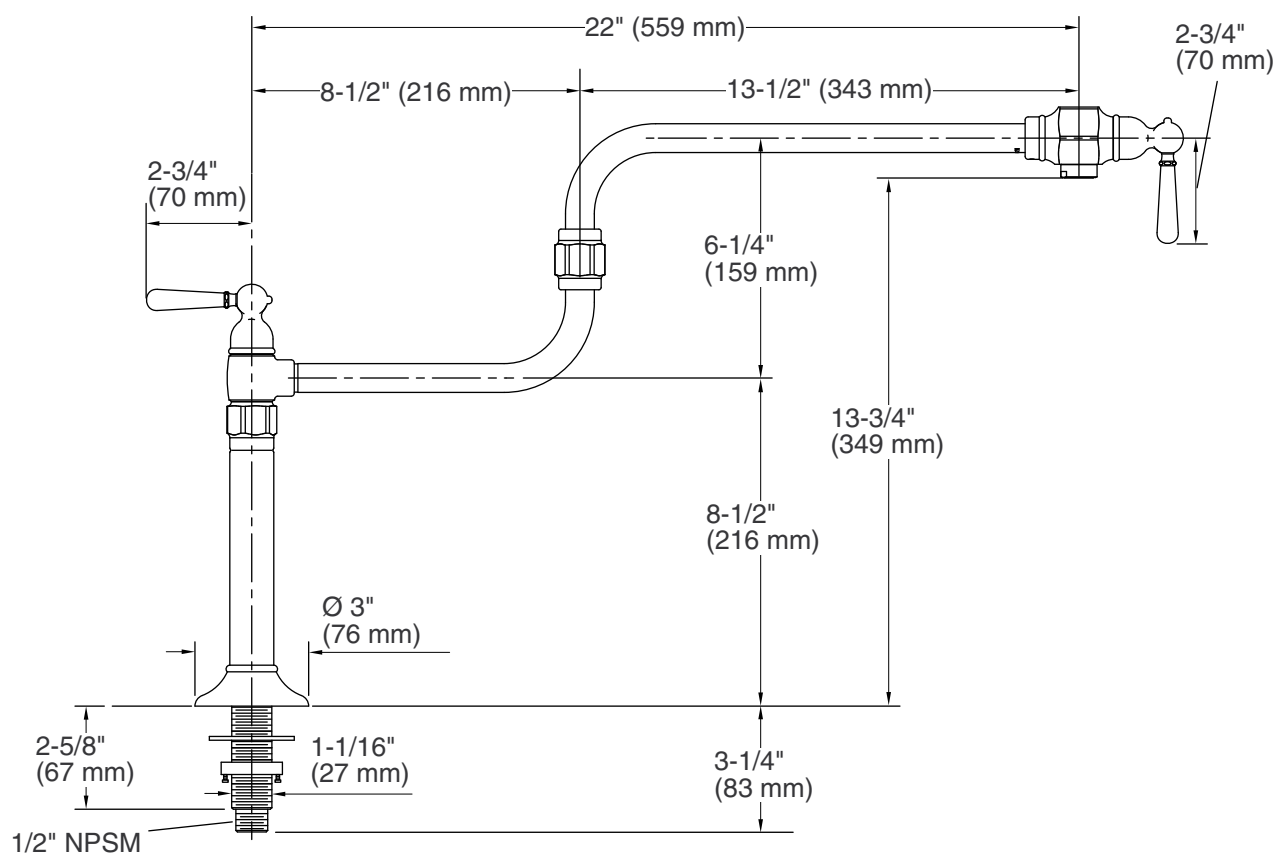
Product Diagram
