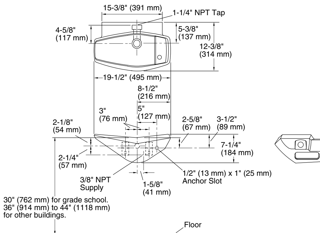
Product Diagram
