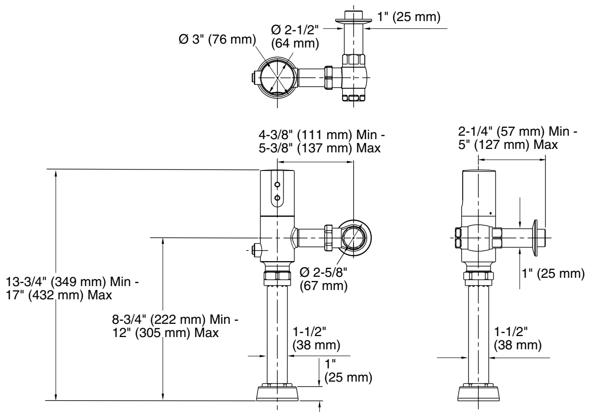
Product Diagram
