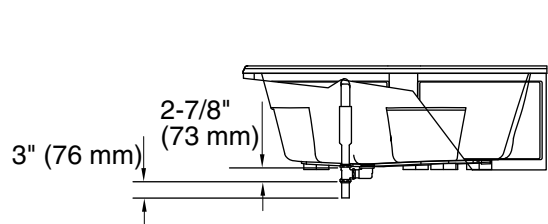
Drop-In Rim Style Cut-Out Detail
